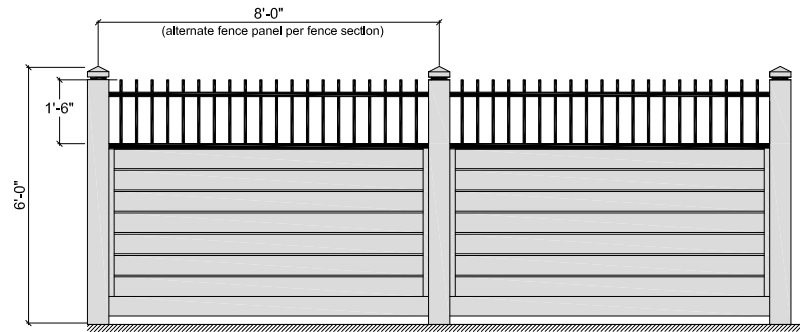
1 Solid Fence with Open Style Top Elevation - Typ. 1 Solid Fence with Wrought Iron Top - NTS
