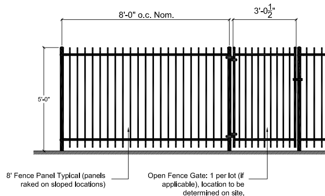
4 Rear Yard Open Fence Elevation - Typ. 1 Open Fence Design - NTS
