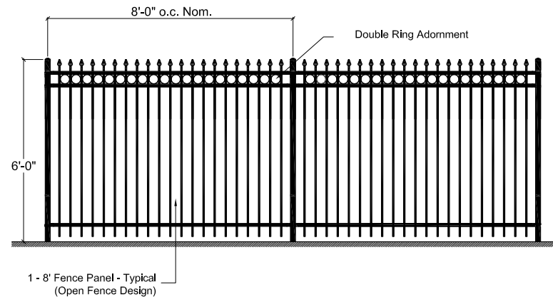
5 Open Fence adjacent to Cemetery Elevation - Typ. 1 Open Fence Design - NTS
